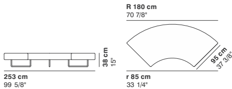
cod. 8467 / bench R 180
