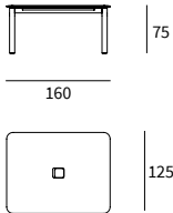
CONFERENCE TABLE P 160X125
