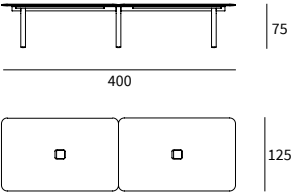
CONFERENCE TABLE 2P 400X125
