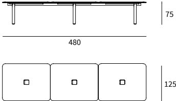
CONFERENCE TABLE 3P 480X125
