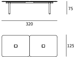
CONFERENCE TABLE 2P 320X125
