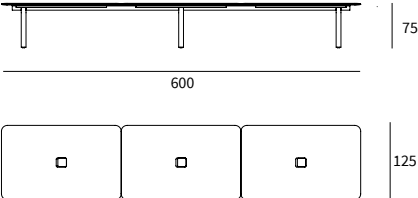
CONFERENCE TABLE 3P 600X125
